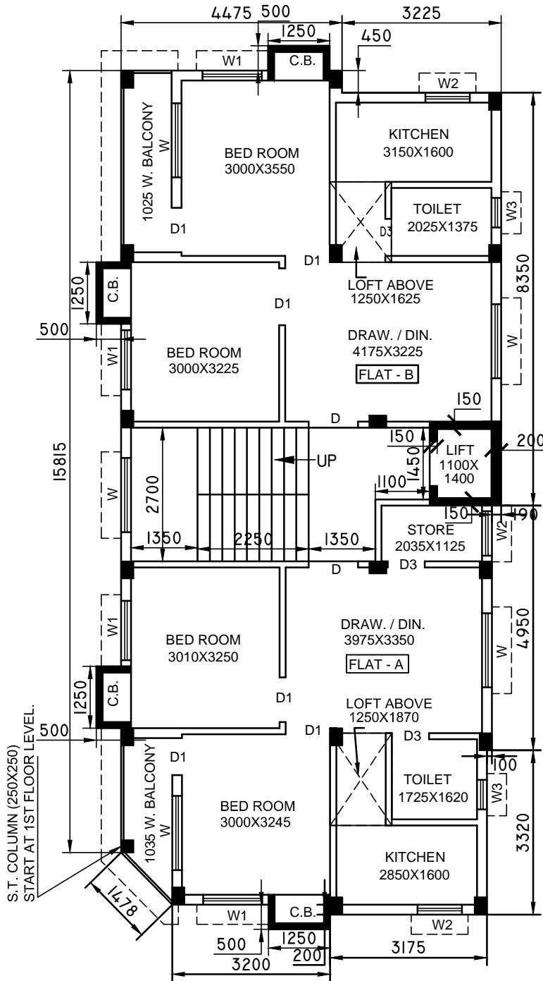
TYPICAL FLOOR PLAN (1ST, 2ND & 3RD)
